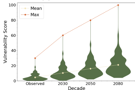
Substation Equipment and Extreme Heat Vulnerability
