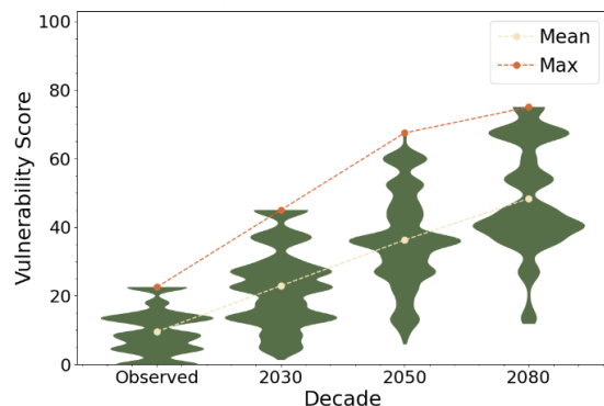
Transmission Spans and Extreme Heat Vulnerability
