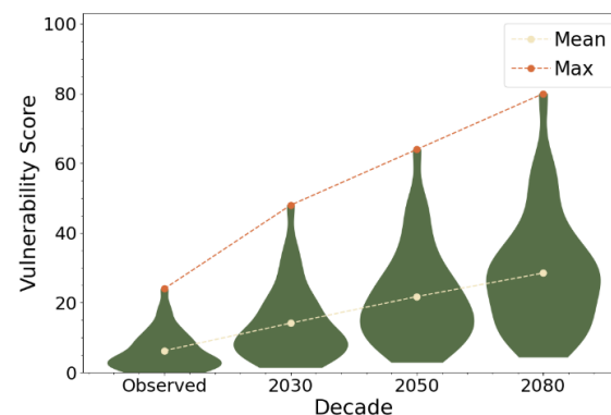
Substation Transformers and Extreme Heat Vulnerability
